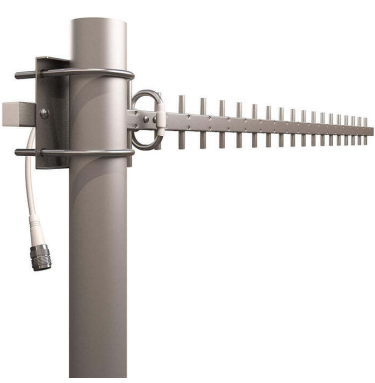
Yagi
